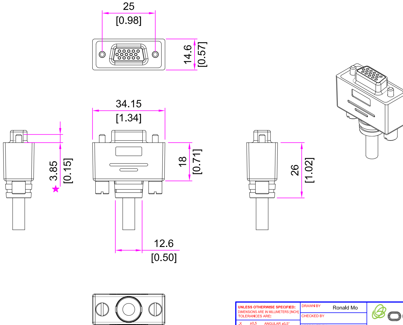
Figure1. Drawing and dimensions
